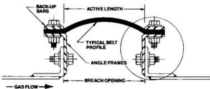
Externally Installed — Bolted Back-Up Bars
