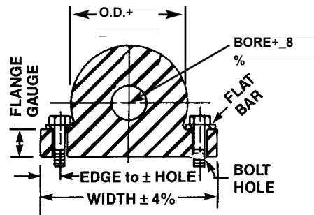
SECTION E-E
